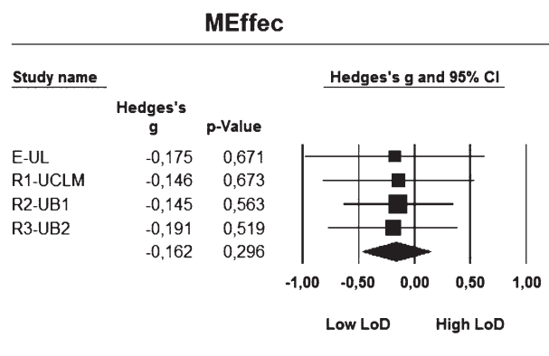
Fig. 6 Meta-analysis of MEffec
